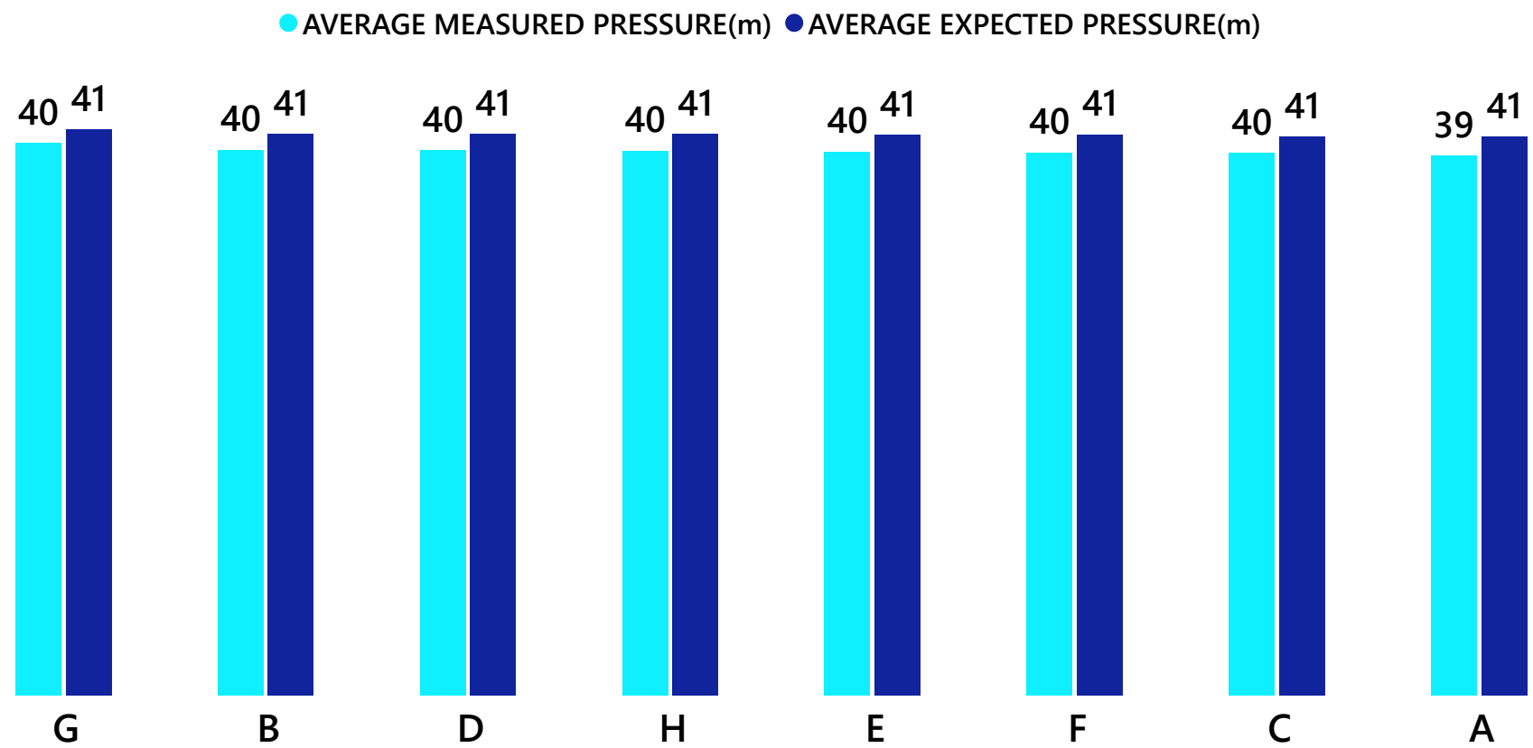
AVERAGE MEASURED PRESSURE V/s AVERAGE EXPECTED PRESSURE PER BLOCK
