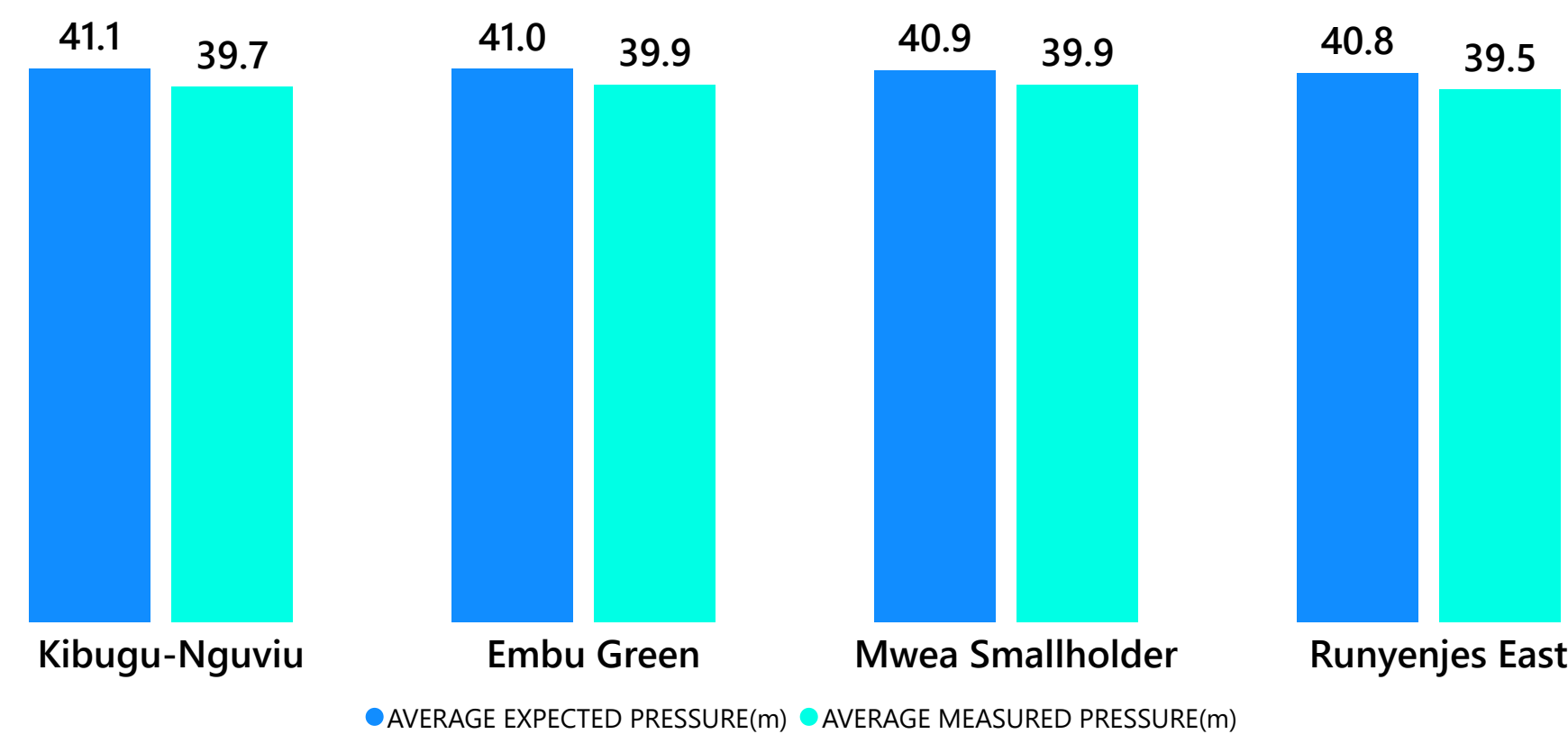
AVERAGE EXPECTED PRESSURE AND AVERAGE MEASURED PRESSURE PER SCHEME
